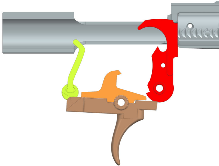
Trigger Member Released Position
