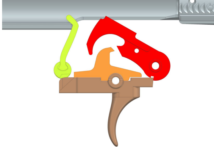
Hammer Set Position
