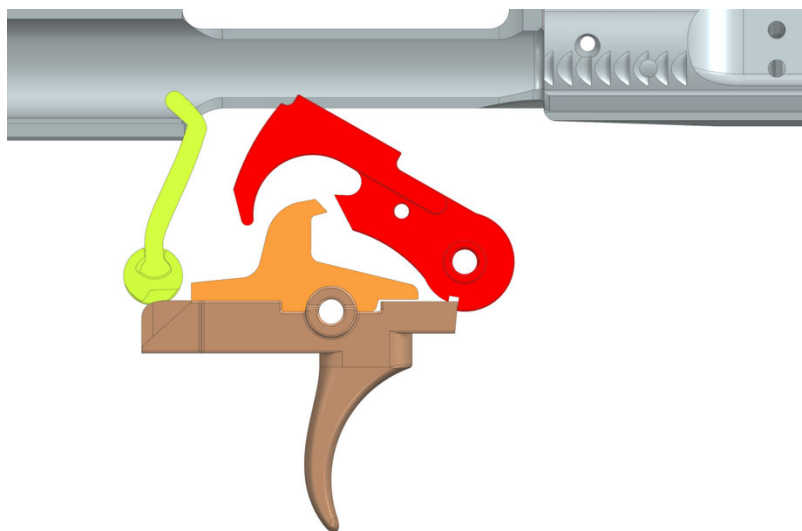
Trigger Member Set Position
